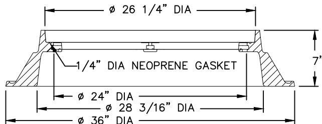
FRAME SECTION
